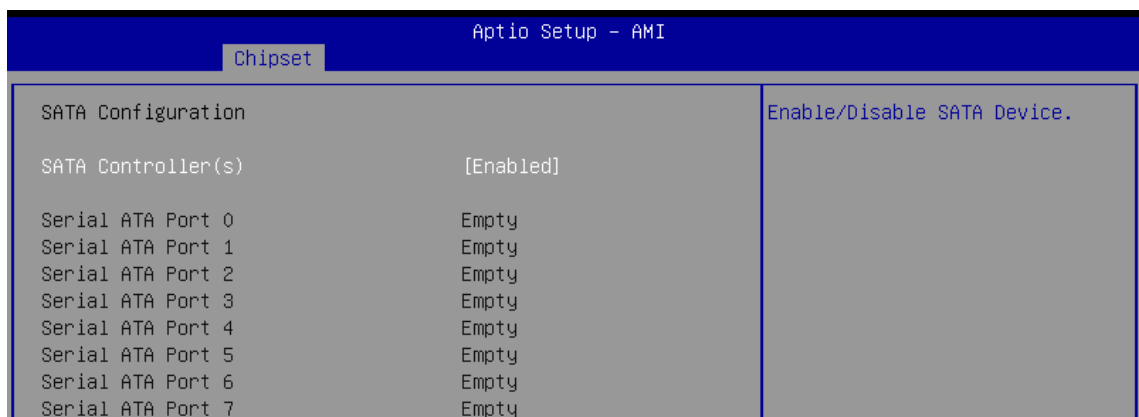
Figure 4-4-2-1: SATA Configuration
