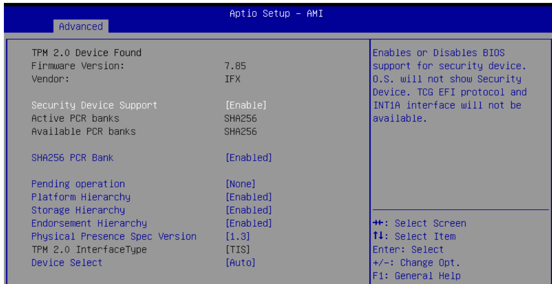
Figure 4 3-3: Trusted Computing
