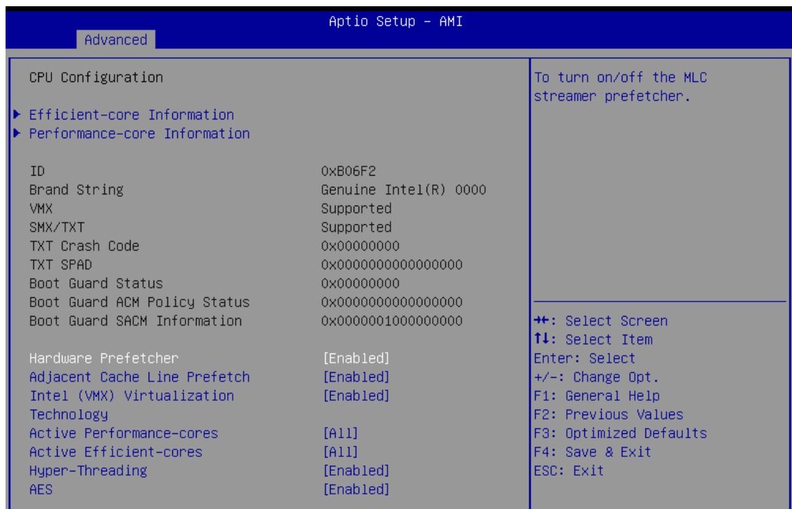
Figure 4 3-1: CPU Configuration
