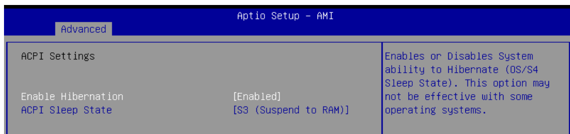
Figure 4 3-4: ACPI Settings
