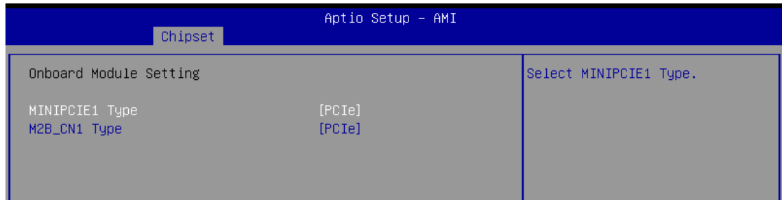
Figure 4-4-3: Module Management
