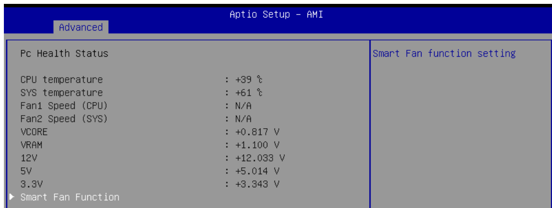
Figure 4-3-6: Hardware Monitor
