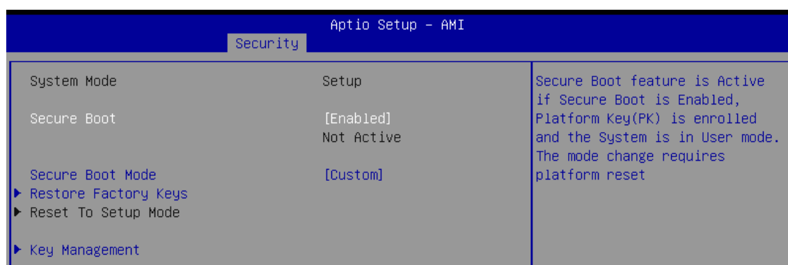
Figure 4-5-2: Secure Boot
