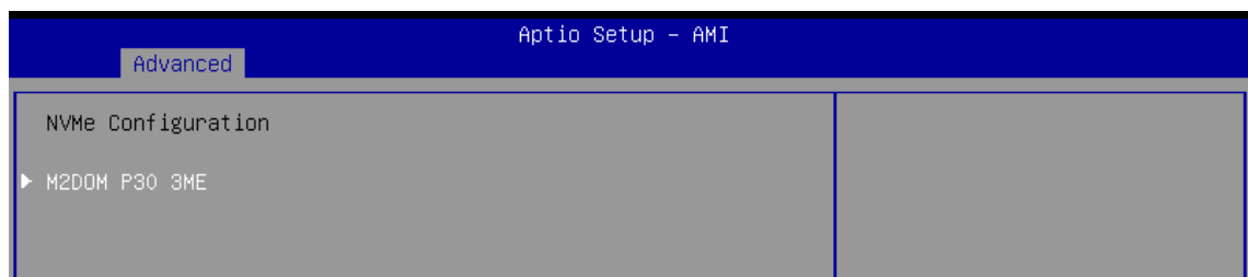
Figure 4-3-8: NVMe Configuration
