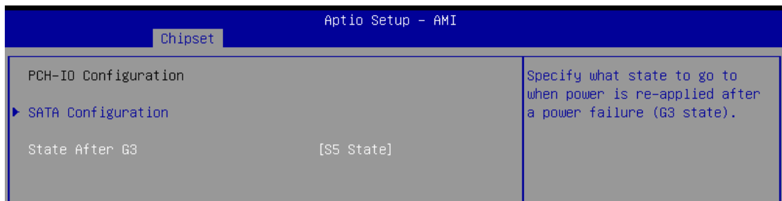
Figure 4-4-2: PCH-IO Configuration
